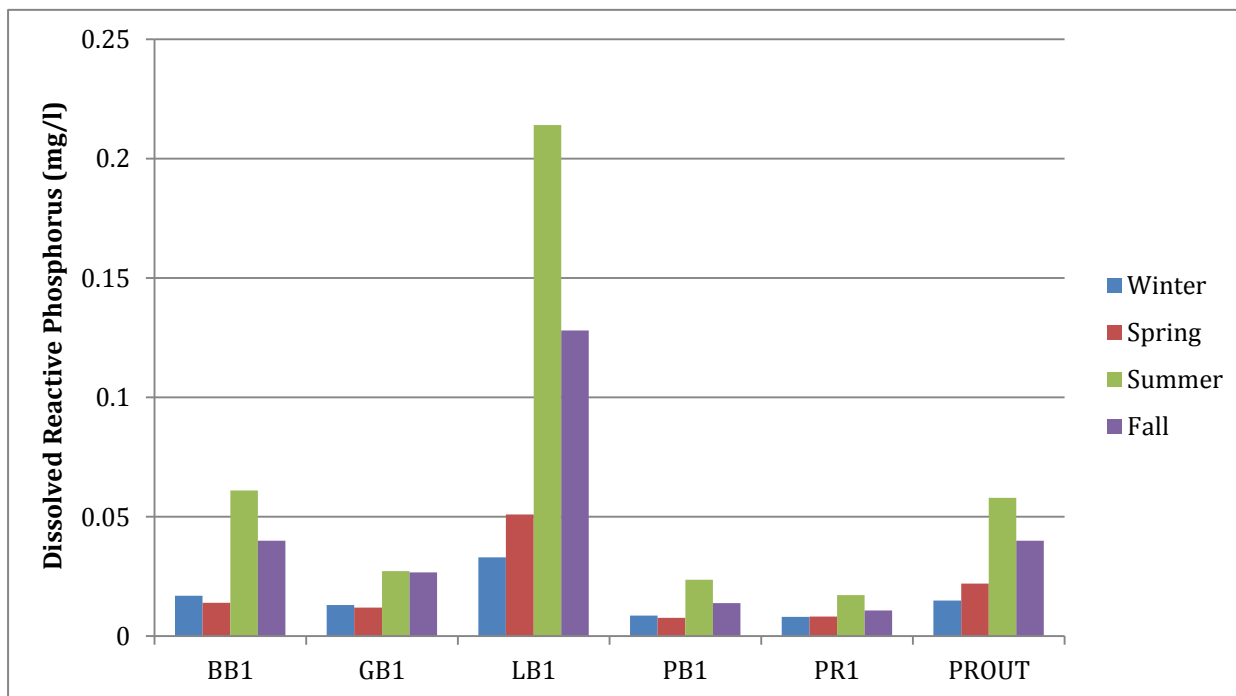
Figure 7. Seasonal Variations of Dissolved Reactive Phosphorus
