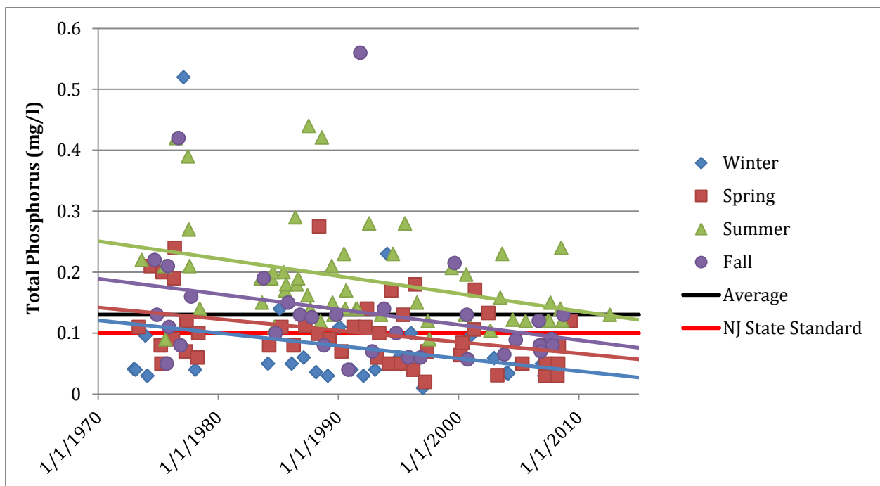
Figure 8. Decreasing Total Phosphorus at PROUT, 1972-2012
