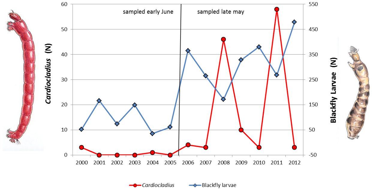
Figure 5. Predator-Prey Relationship at Great Brook Macroinvertebrate Sites
