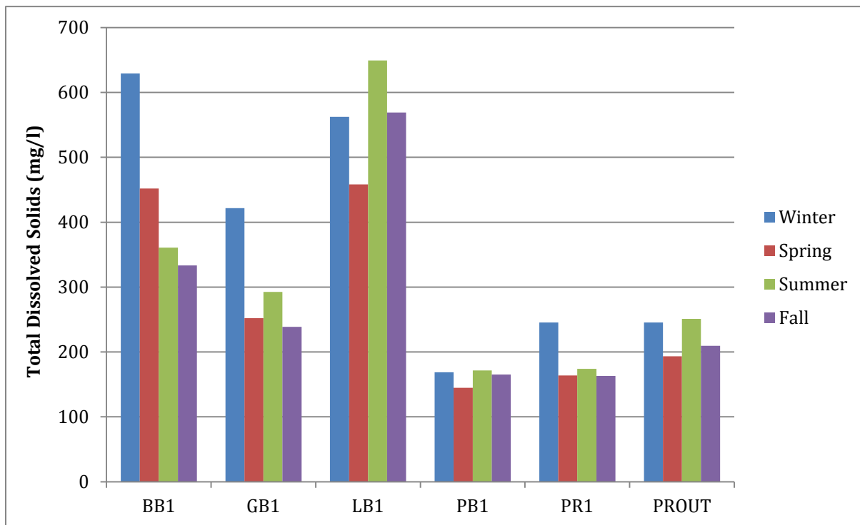
Figure 11. Seasonal Variations of Total Dissolved Solids
