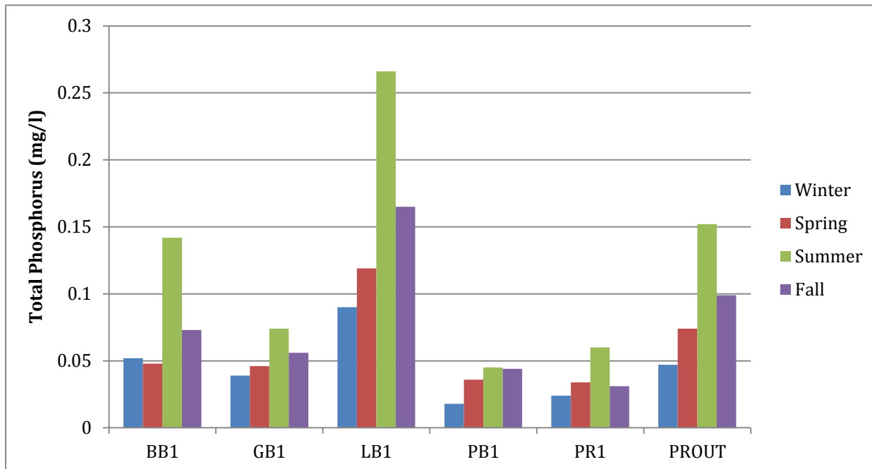
Figure 6. Seasonal Variation of Total Phosphorus
