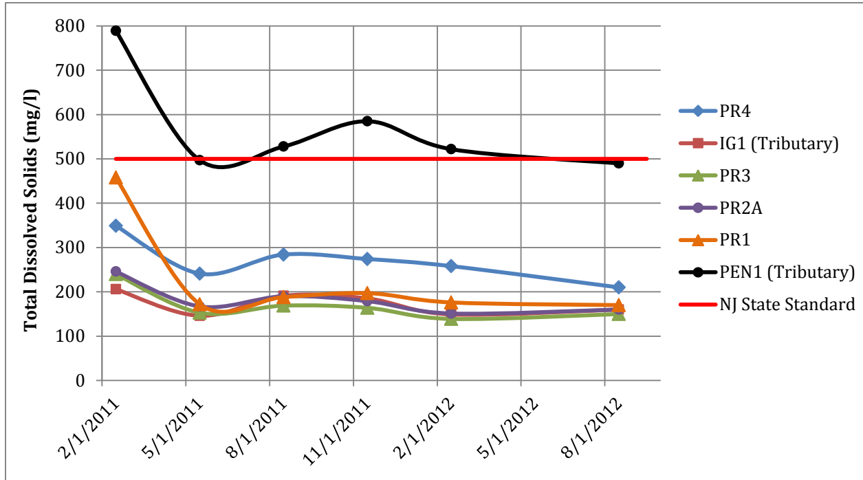
Figure 13. Impact of Snow on Total Dissolved Solids
