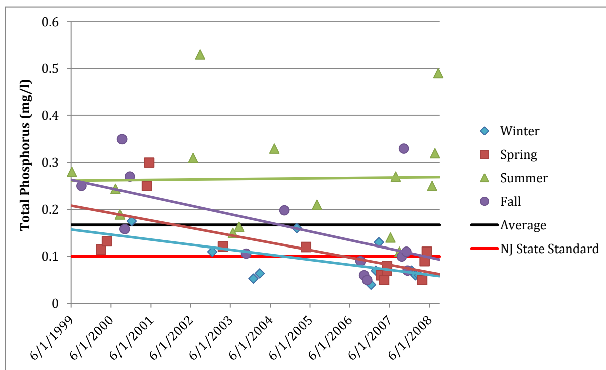
Figure 9. Seasonal Total Phosphorus Trends at LB1
